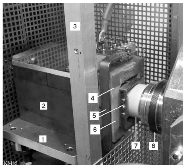
Fig. 4: Photograph of the kicker magnet. 1: adjustable base plate, 2: ferrite yoke, 3: partially opened shielding cage, 4: upper coil, 5: current leads, 6: lower coil, 7: ceramic vacuum tube, 8: bellows. See also reference [2].
