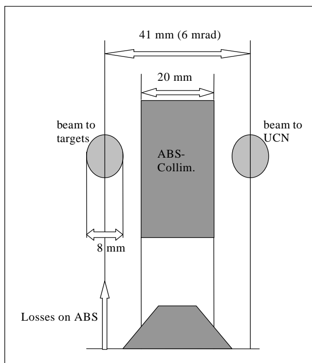
Fig. 3: The beam situation in front of the magnetic septum magnet (ABS). If the transition with time were linear, then about 50 % of the beam spill produced by the 6-mrad-kick would be deposited on the purely radiation-cooled ABS tungsten collimator. The width of the collimator is 20 mm and the beam separation ca. 41 mm. The 4\sigma width of the 2 mA proton beam is expected to be about 8 mm. The 20 mm sweep over the collimator is done within 200 \mu s [1].
