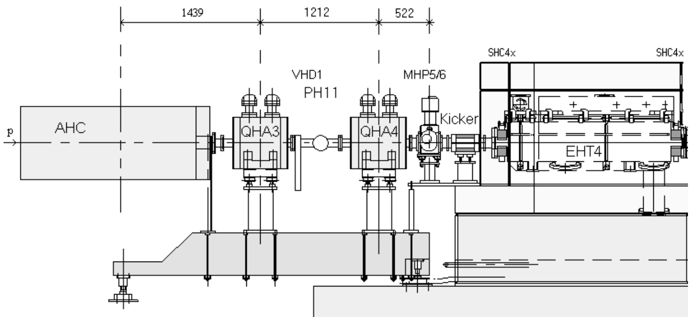
Fig. 1: New layout of the section of the proton beam line for switching with the fast kicker magnet. AHC: bending magnet; QHA3/4: quadrupole lenses, PH11: vacuum pump; VHD1: vacuum valve; MHP5/6: beam monitors; EHT4: electrostatic beam splitter; SHC4x: steering magnets; Kicker: newly installed fast deflecting magnet [2].
