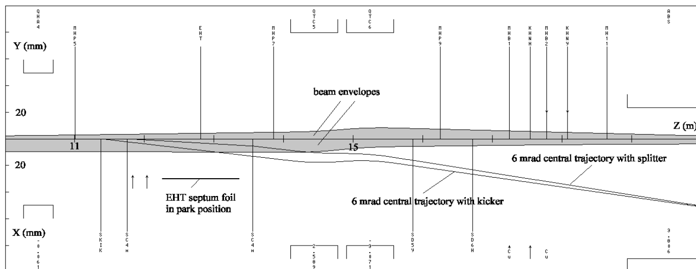
Fig. 2: The kicked and the statically deflected proton beam central trajectories (6 mrad deflection angle) together with the x- and y-beam envelopes ( 2\sigma ). The kicked beam will produce larger losses at the parked septum foil than the statically deflected beam.
