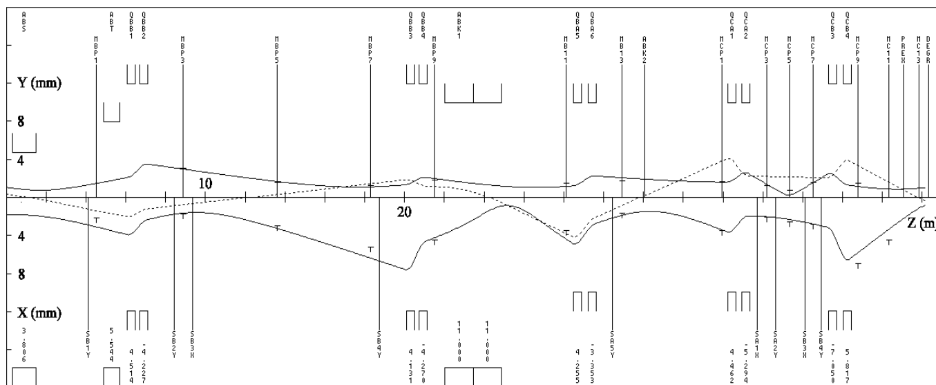
Fig. 5: Envelope fit with the measured beam profile widths of the kicked proton beam at 20 \mu\text{A} intensity. The measured 2\sigma -widths are marked with \perp and T, whereas the solid curves represent the fitted x- and y-envelopes. The dotted line is an assumed 1-permille-dispersion trajectory. Per kick only 3 to 4 profiles could be recorded. Therefore 7 runs with a waiting time of about 15 minutes in between were needed to gather the required data.
