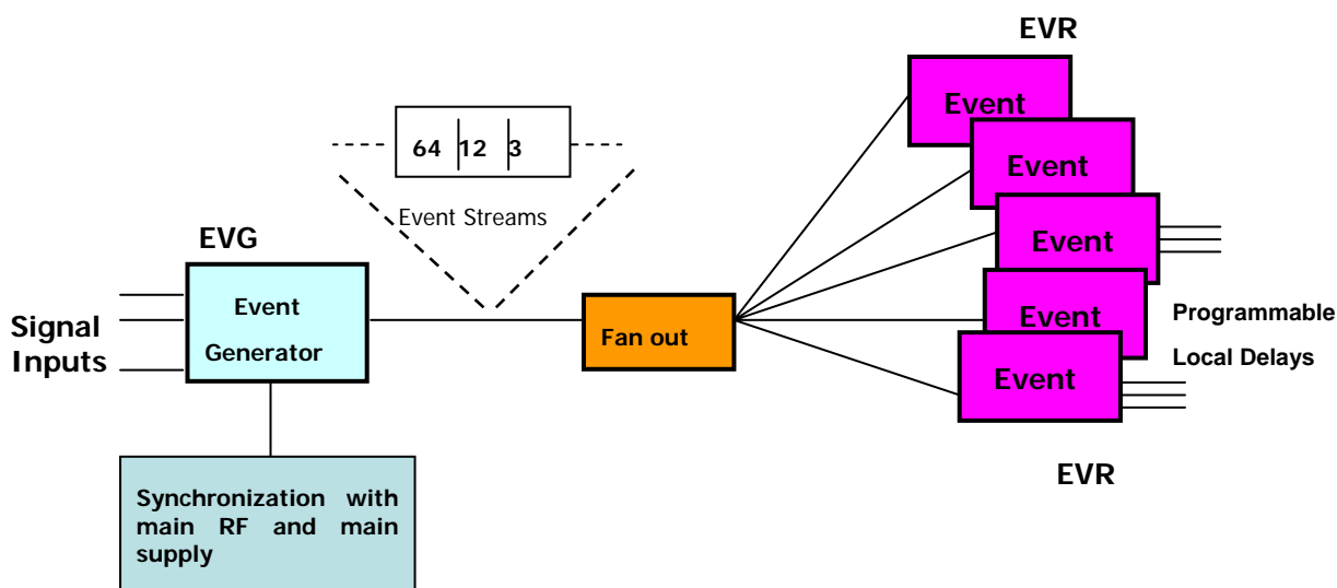
Fig. 1: Global event system architecture.
