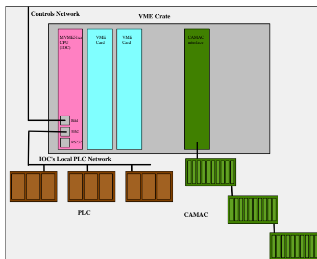
Fig. 1: The new IOC hardware configuration
