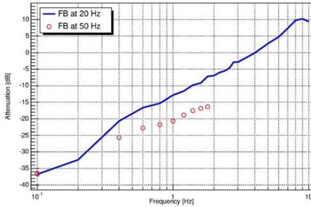
Feedback attenuation
