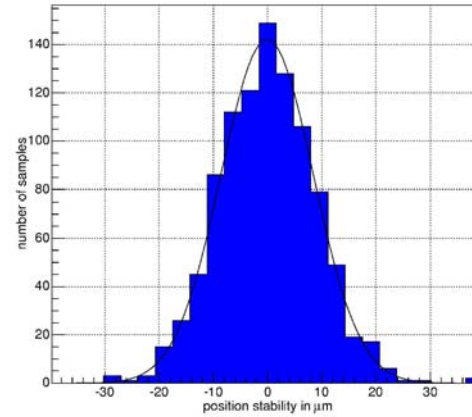
Position distribution @ 100 Hz \sigma = 8.5 \mu\text{m}
